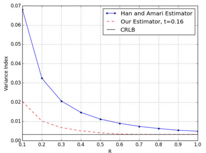
Fig. 8. Performance Comparison: \theta = 0.01 , M = 4 , t = 0.16 .
