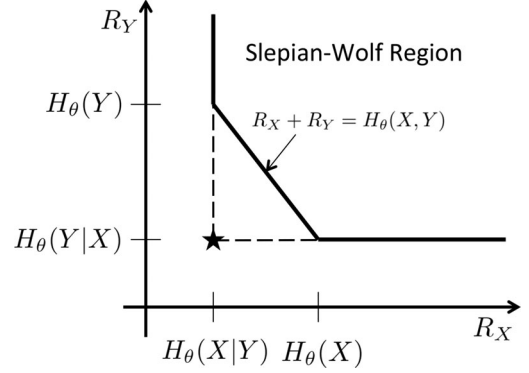
Fig. 2. Our estimator is optimal at any rate larger than the rate pair indicated by (★), which is outside of the Slepian-Wolf rate region.
