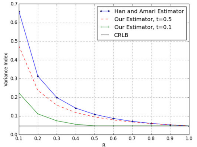
Fig. 7. Performance Comparison: \theta = 0.05 , M = 2 , t = 0.5 and 0.1 .
