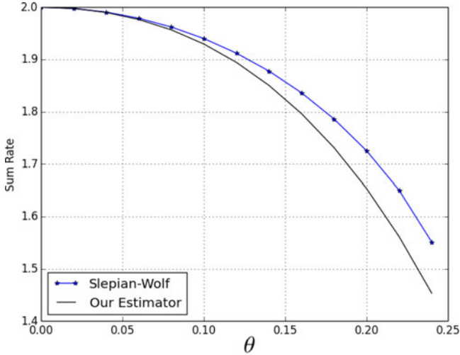
Fig. 3. The required rates to achieve the optimal centralized performance for the binary source given in Table II is lower than Slepian-Wolf rates.
